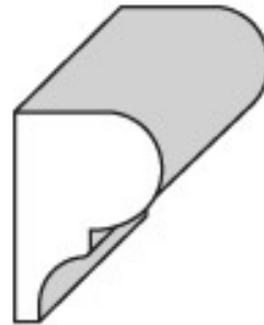
CMK 469 3/4" x 1-1/16"
