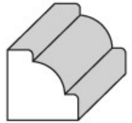
CMK 470 13/16" x 13/16"
